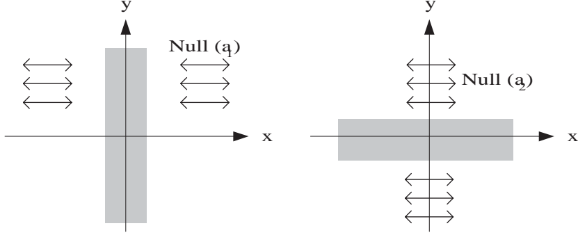
Figure 2: Degenerate Quadratic Forms
